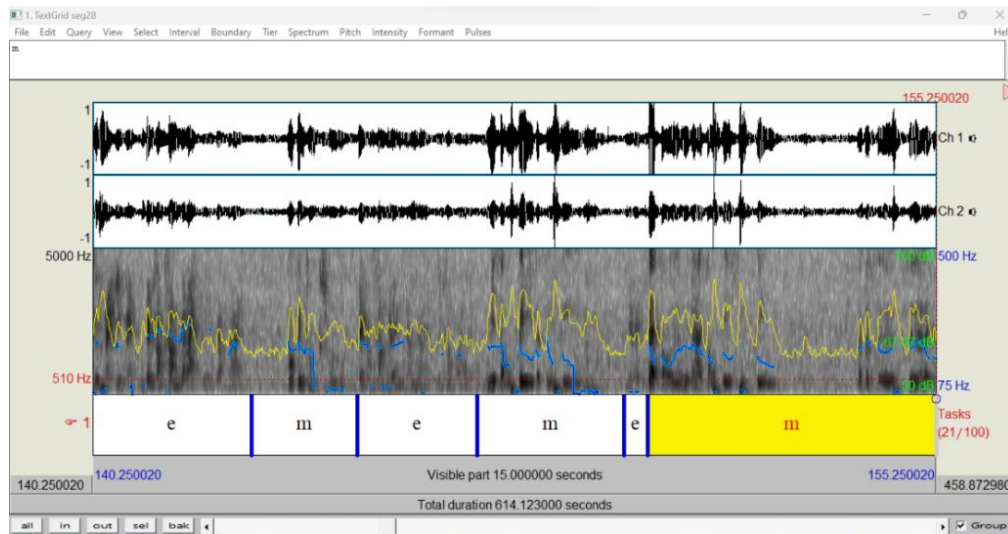
Figure 14 Speaker segmentation
